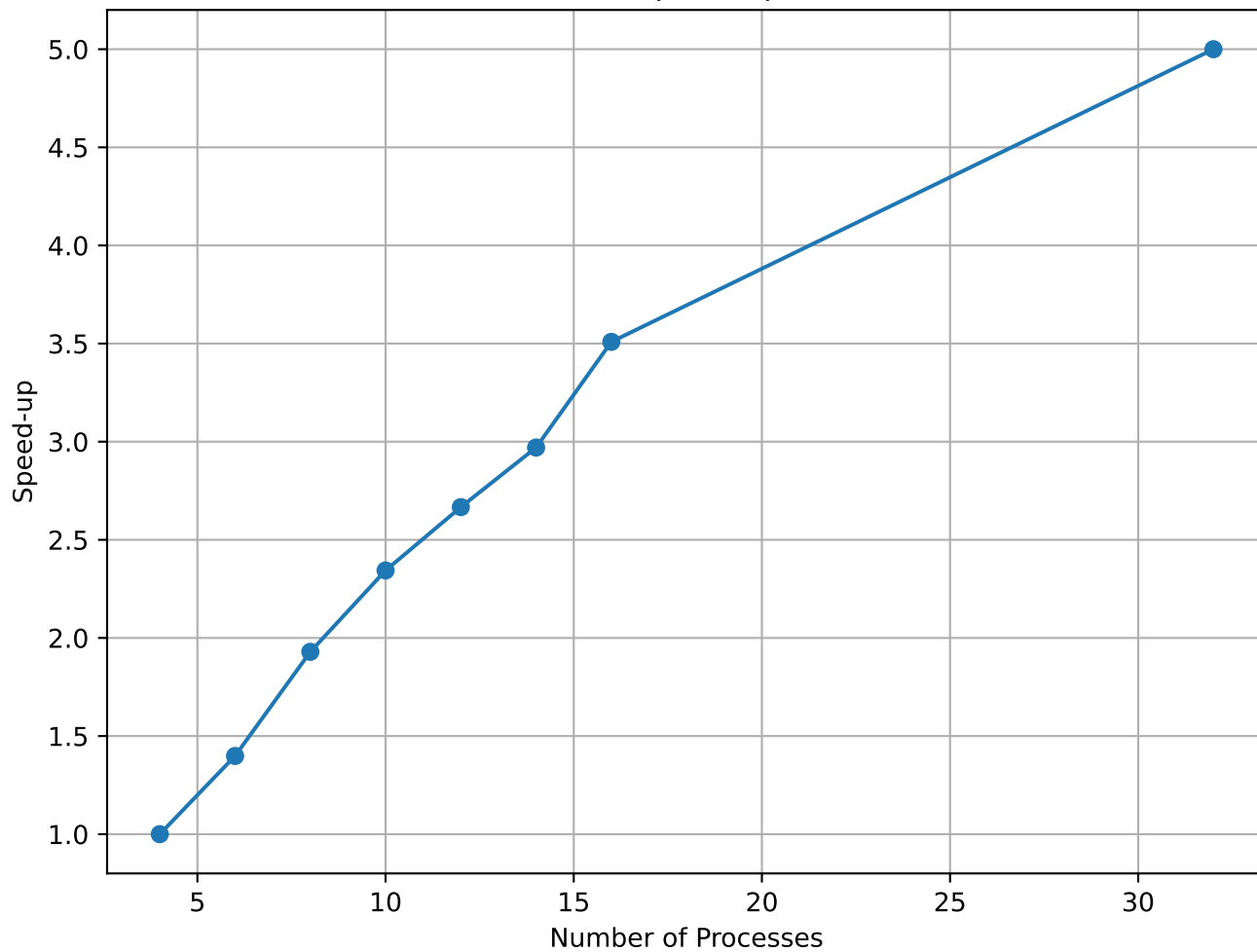
Preconditioner Speed-up (3D harder)
