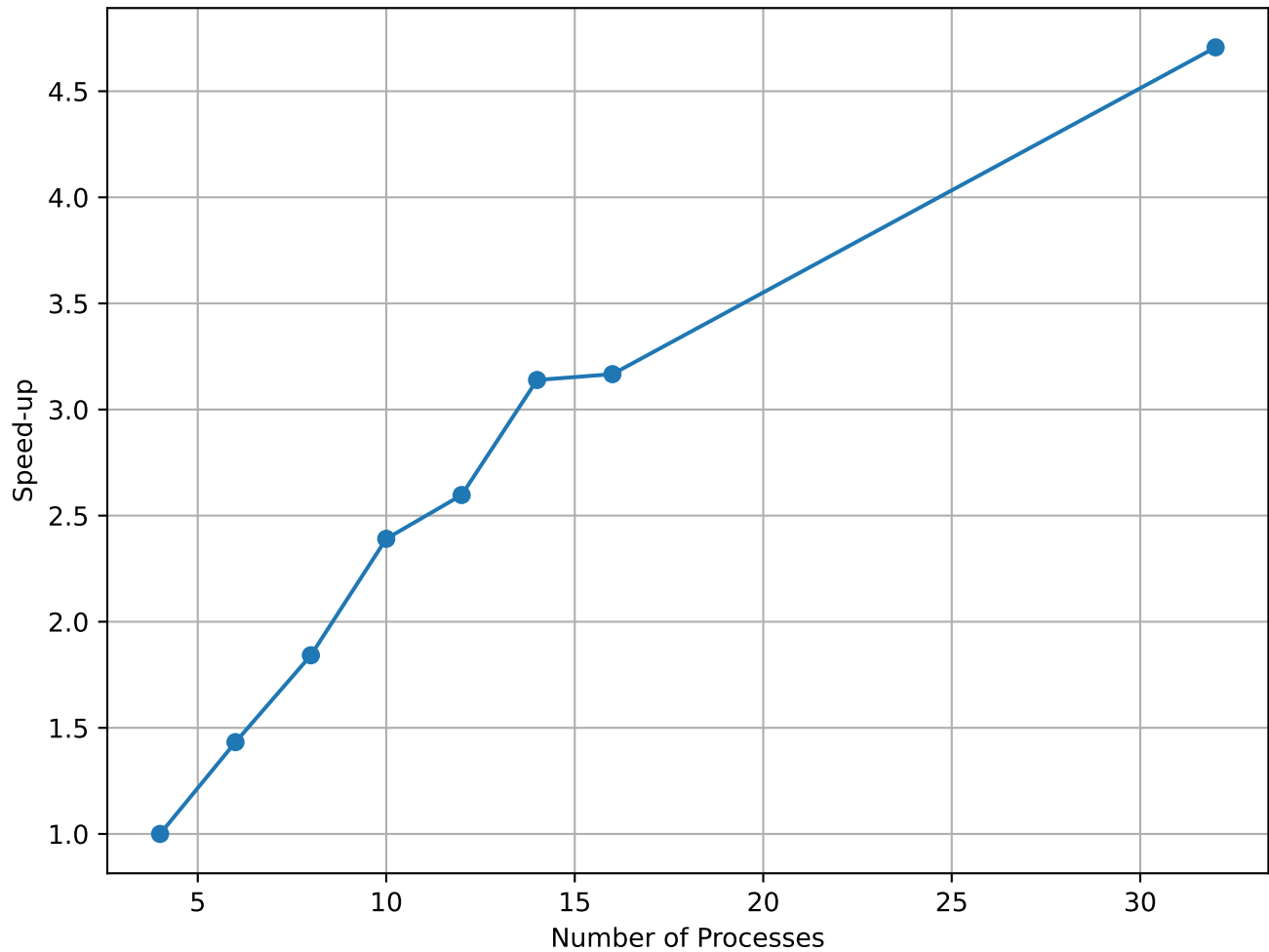
Solve Speed-up (3D harder)
