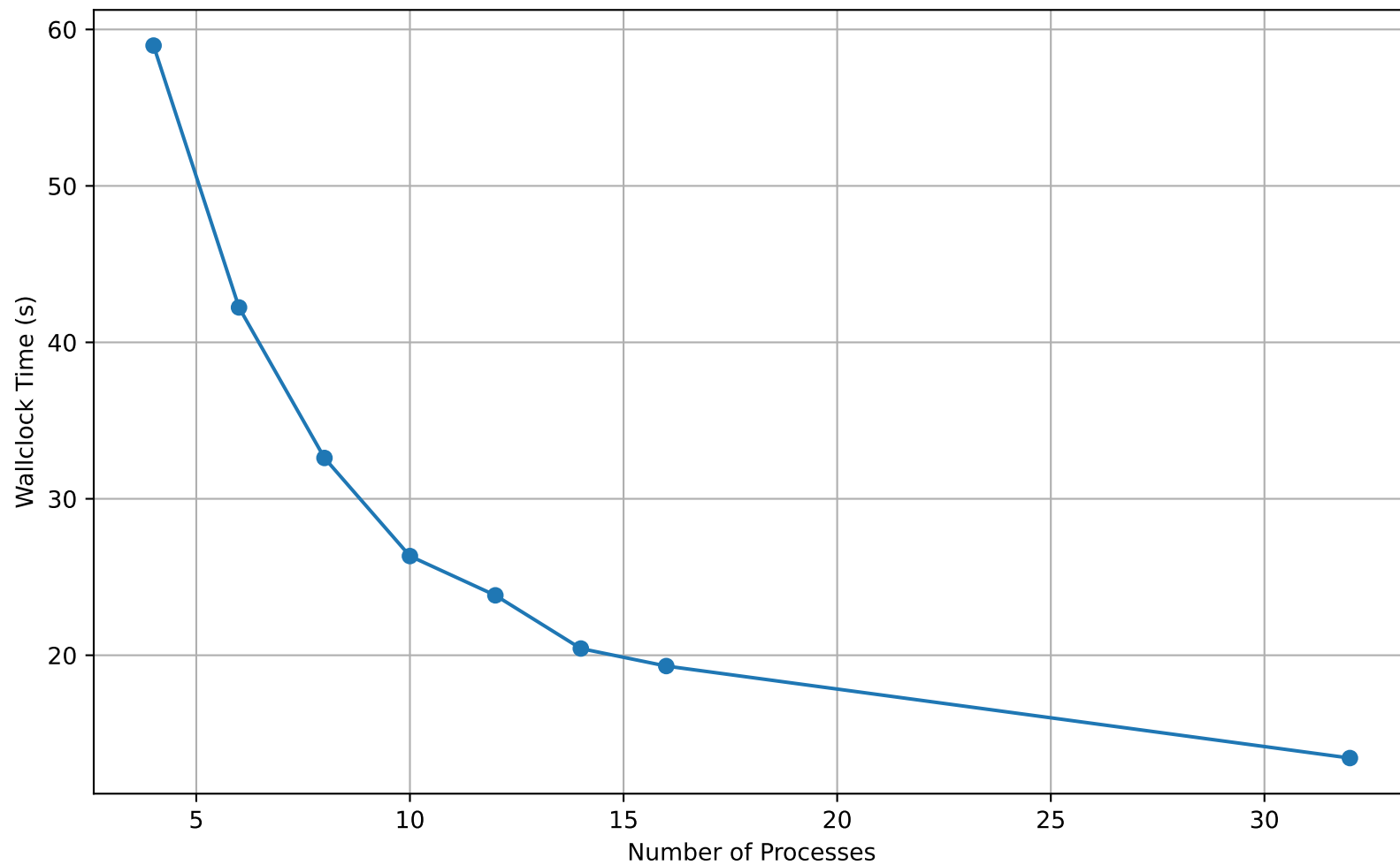
Wallclock Time vs Processes (3D harder)
