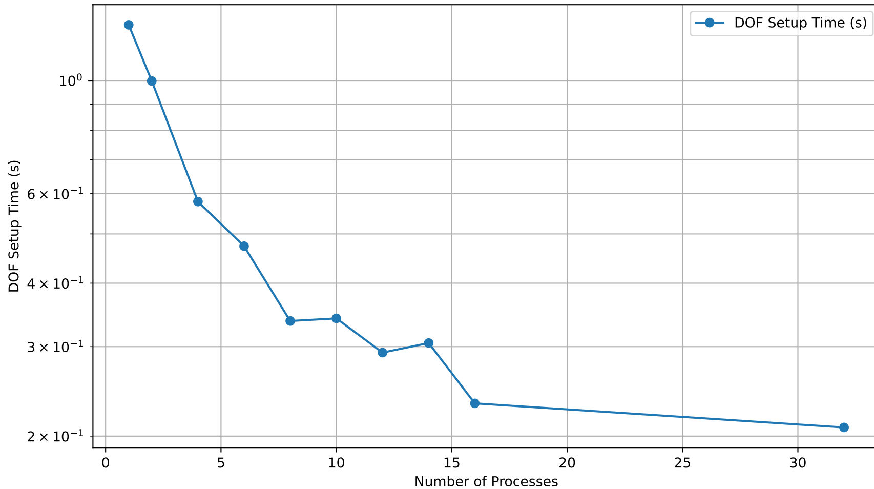
DOF Setup Time vs Number of Processes (3D, no refinement)
