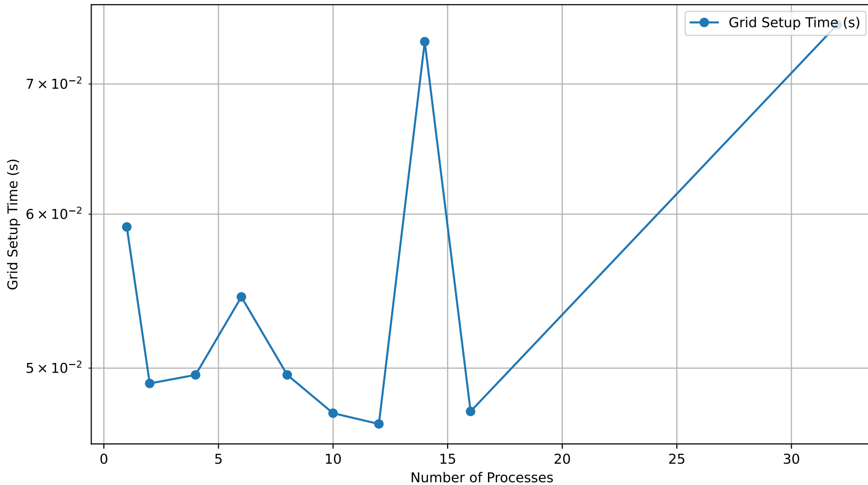
Grid Setup Time vs Number of Processes (3D, no refinement)
