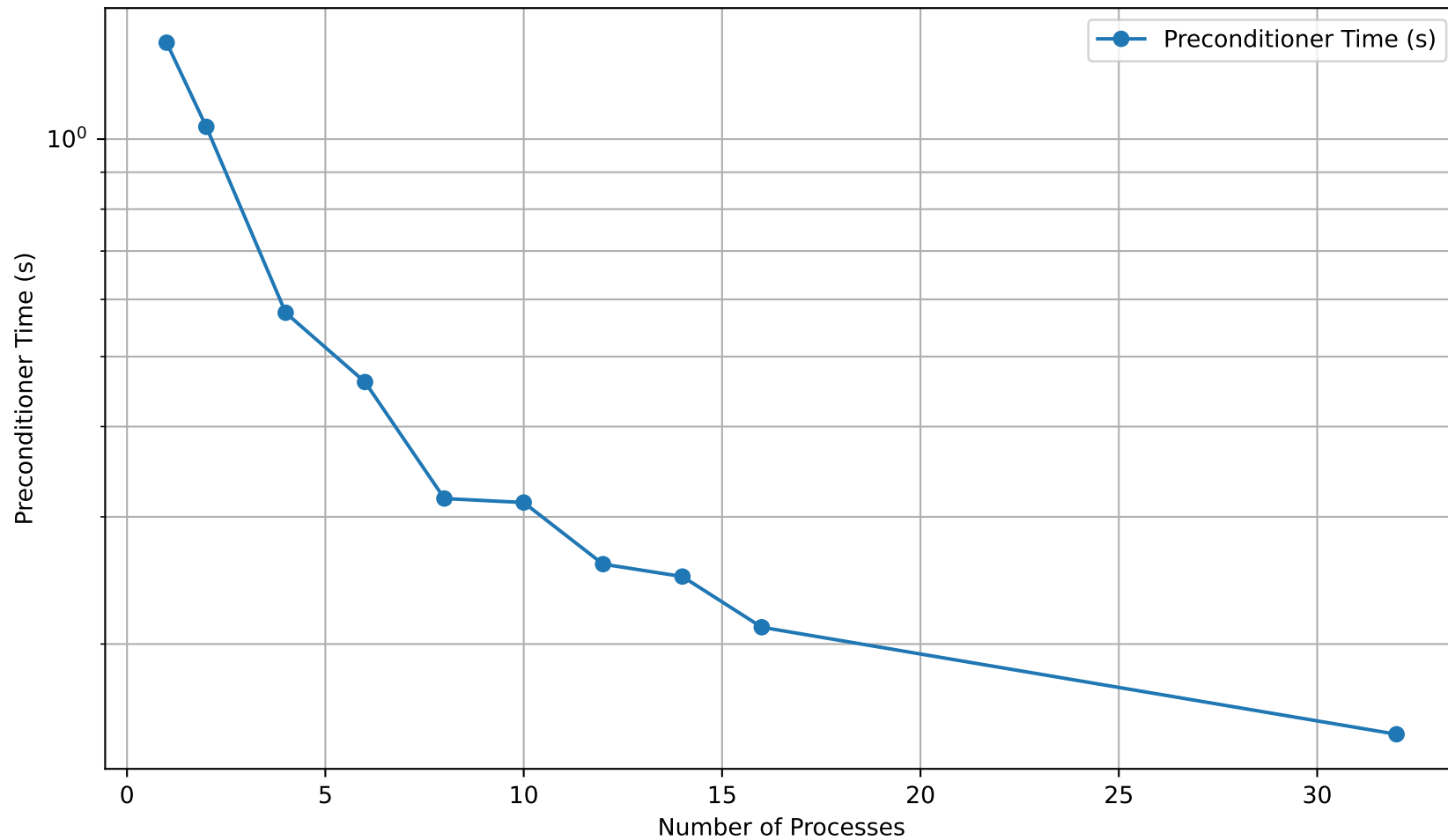
Preconditioner Time vs Number of Processes (3D, no refinement)
