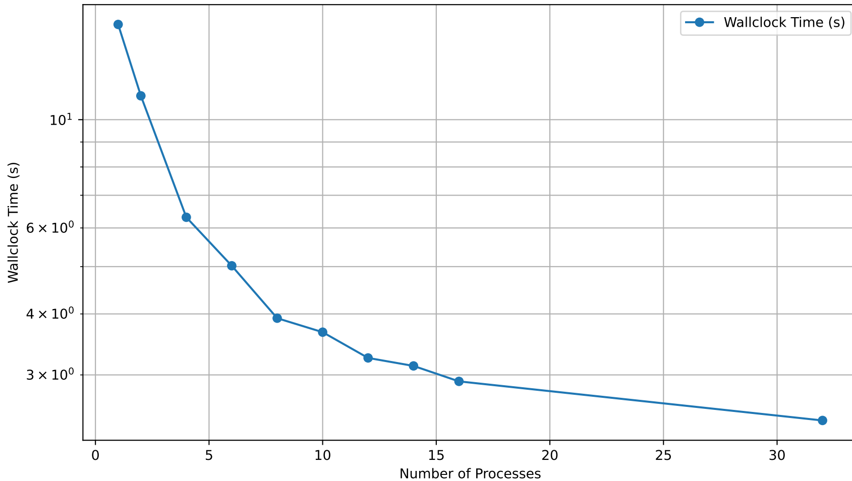
Wallclock Time vs Number of Processes (3D, no refinement)
