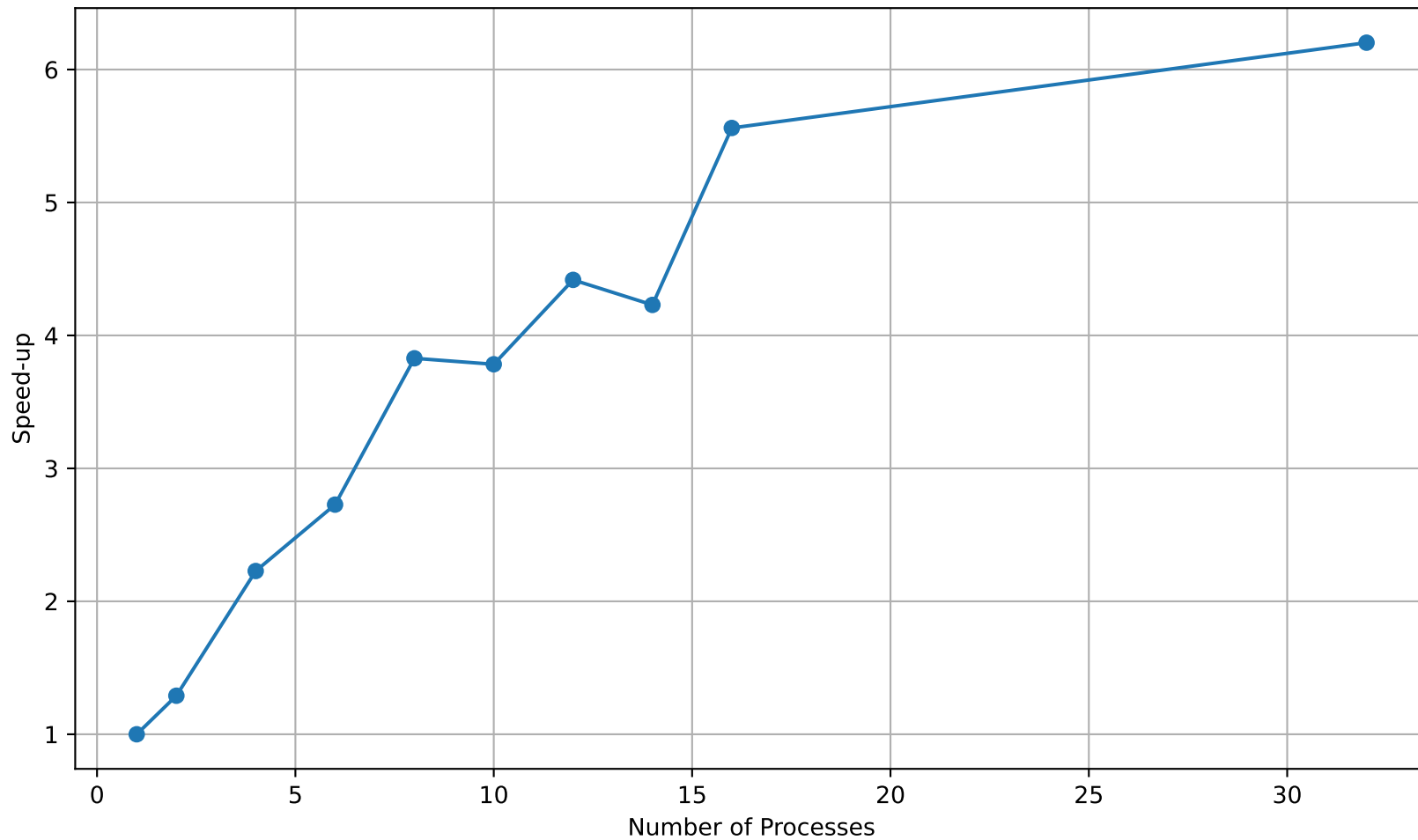
DOF Setup Speed-up (3D, no refinement)
