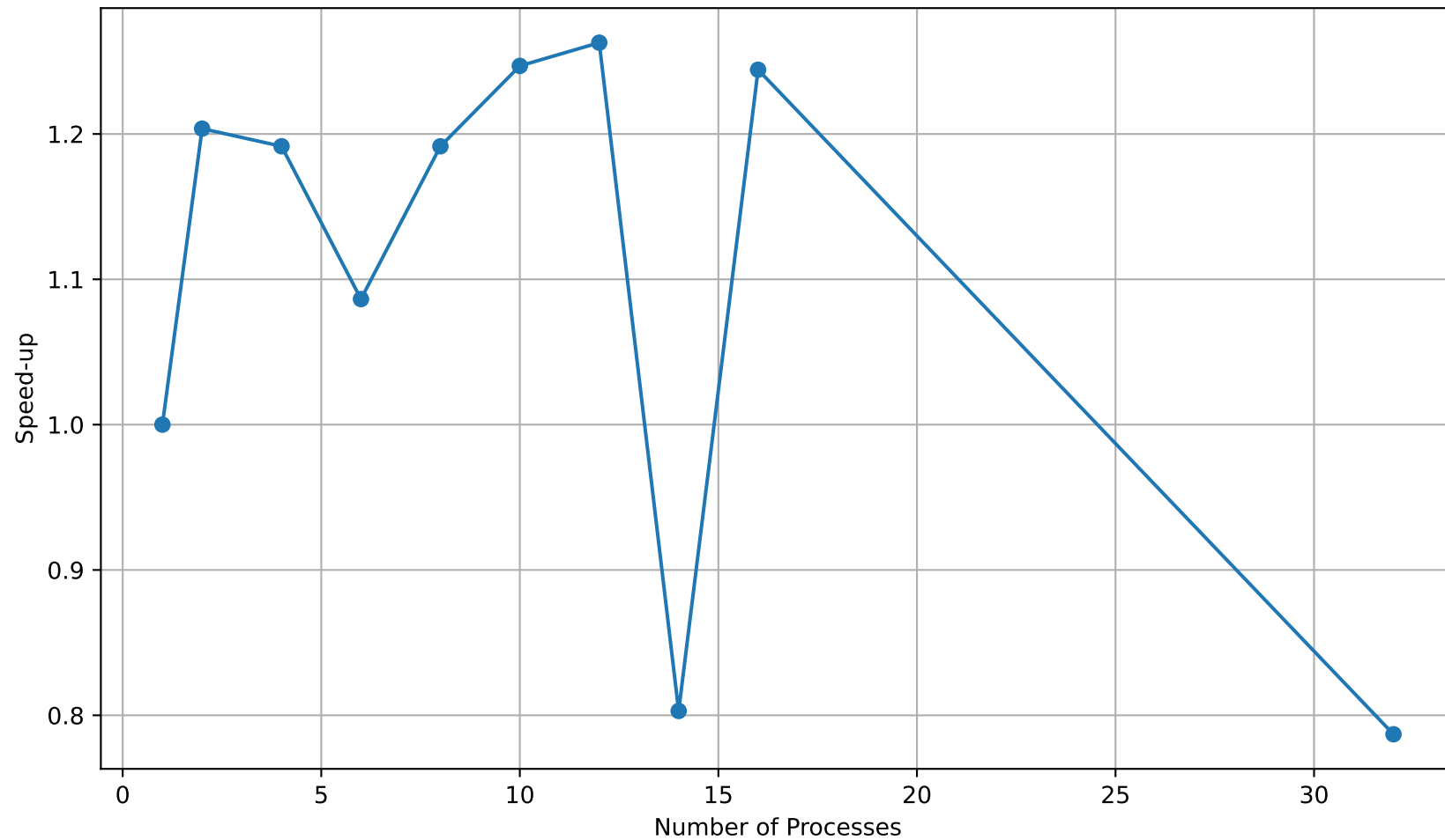
Grid Setup Speed-up (3D, no refinement)
