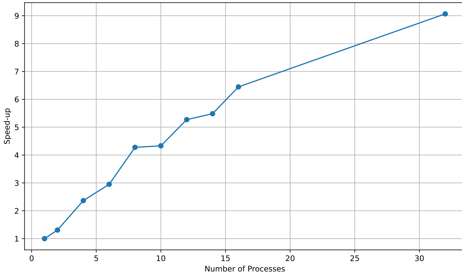
Preconditioner Speed-up (3D, no refinement)
