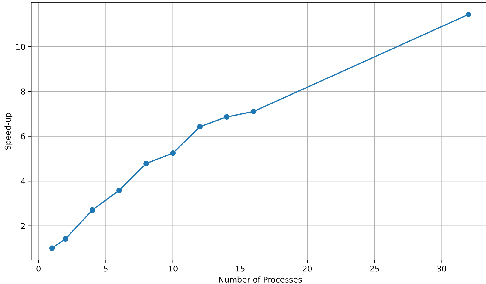
Solve Speed-up (3D, no refinement)
