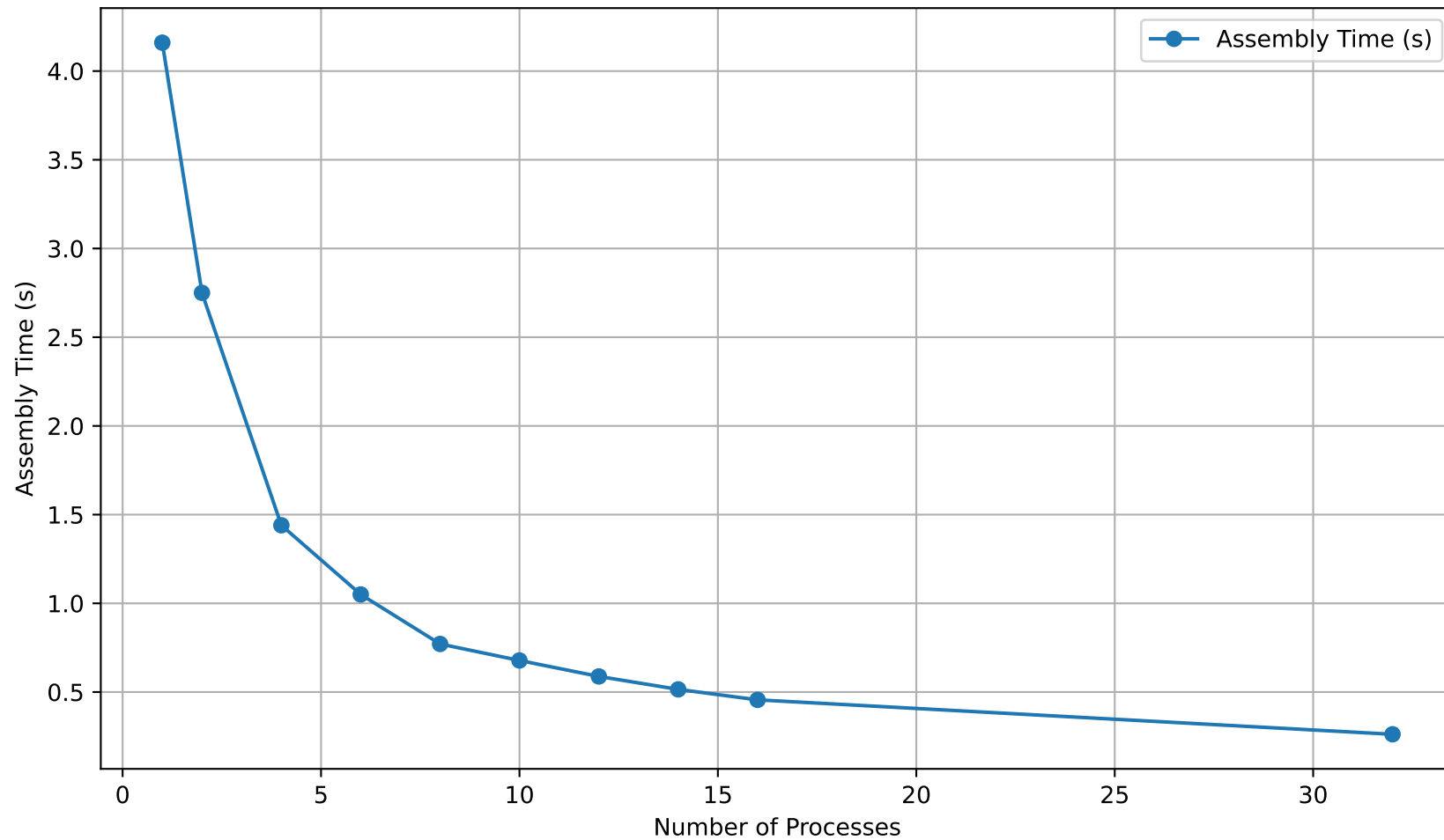
Assembly Time vs Number of Processes (3D, no refinement)
