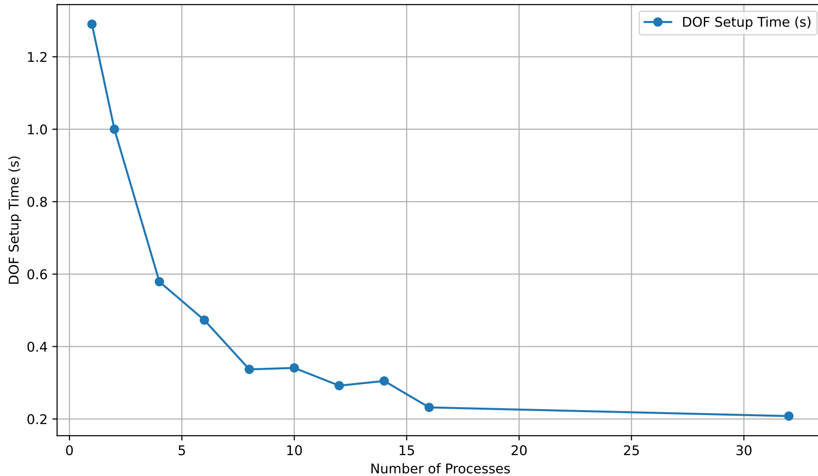
DOF Setup Time vs Number of Processes (3D, no refinement)
