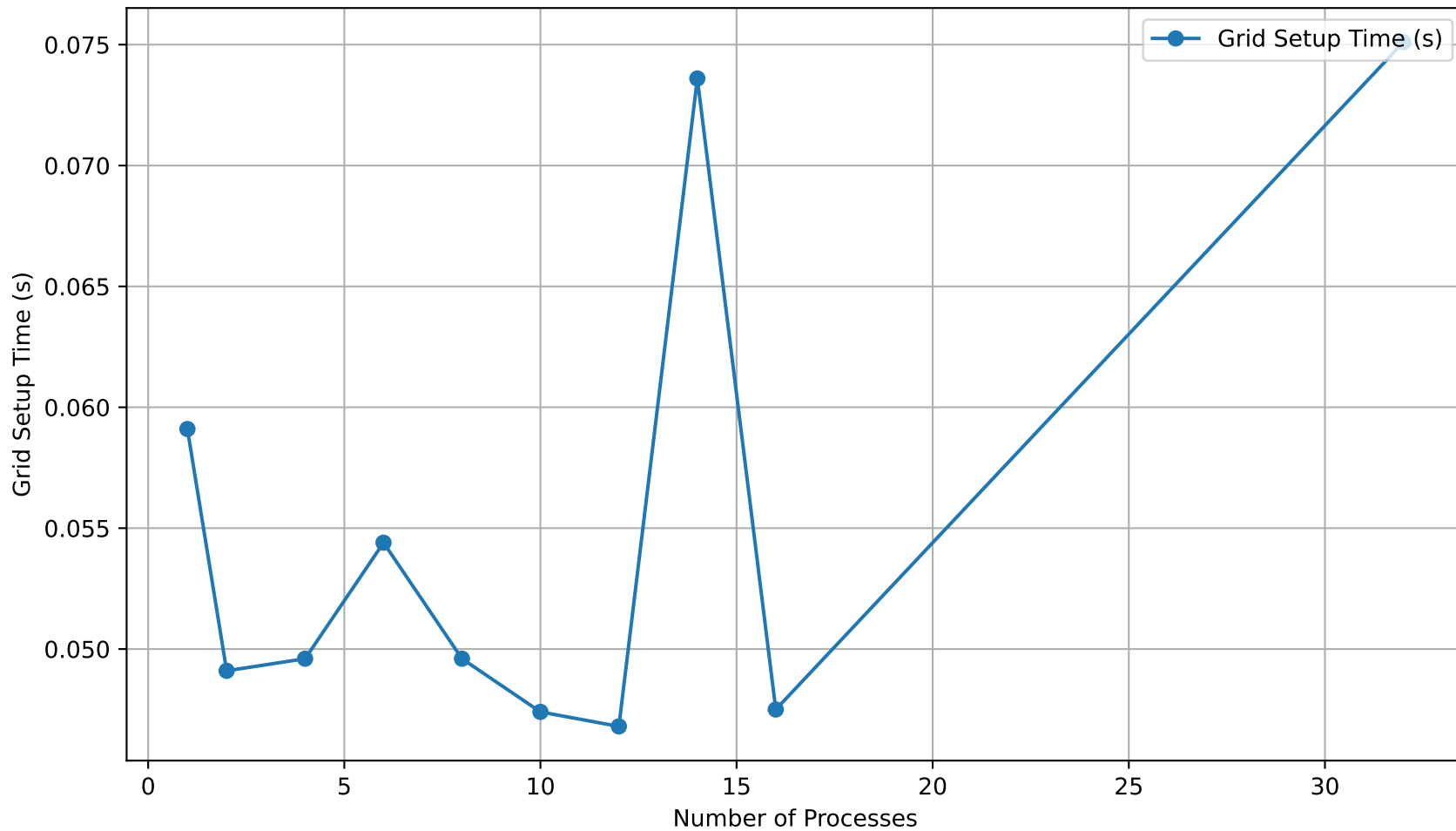
Grid Setup Time vs Number of Processes (3D, no refinement)
