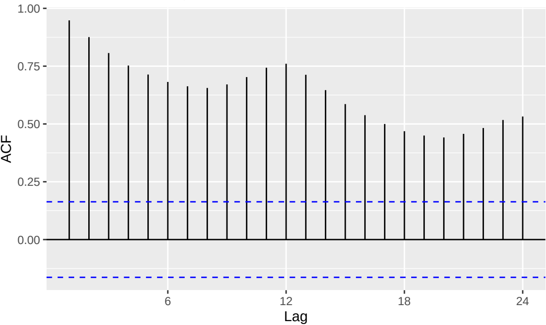
Series: AirPassengers
