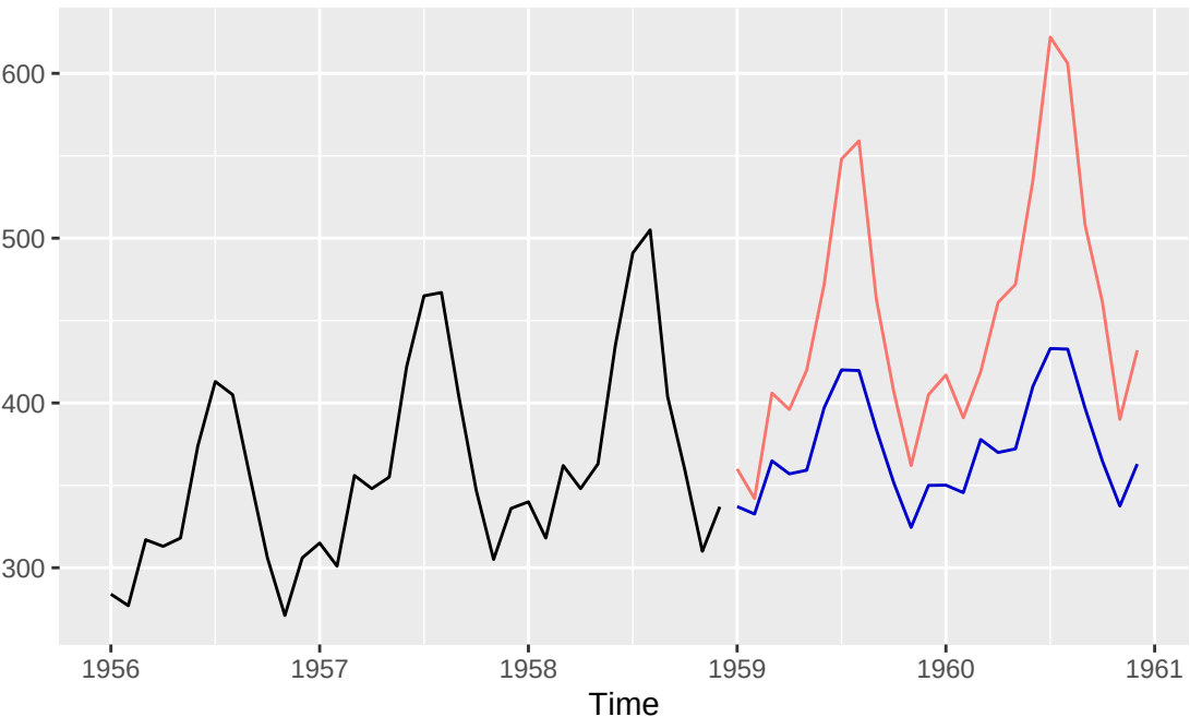
Holt-Winters additivo, serie AirPassengers
