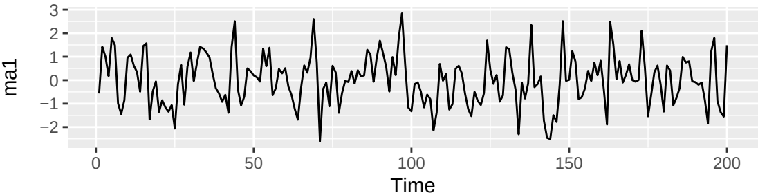
MA(1)
