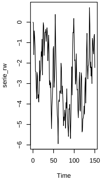
Random walk
