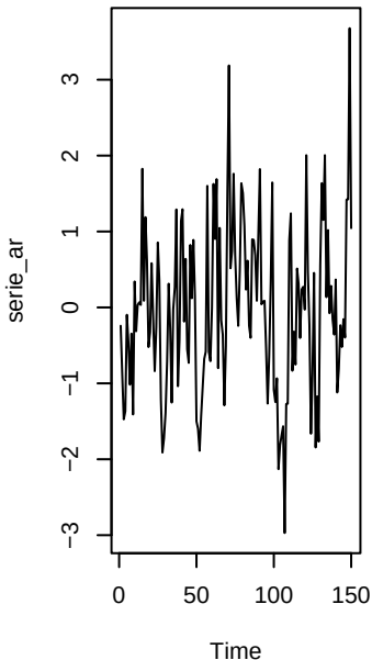
AR(1), alpha=0.5
