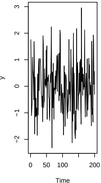
AR(1), \alpha=0.2
