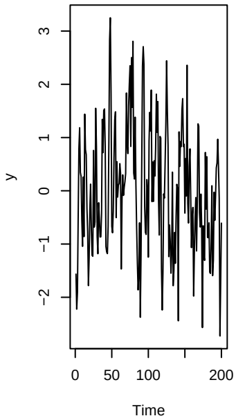
AR(1), \alpha=0.6
