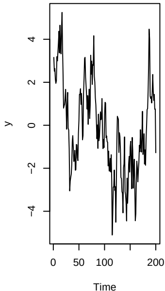
AR(1), \alpha=0.9
