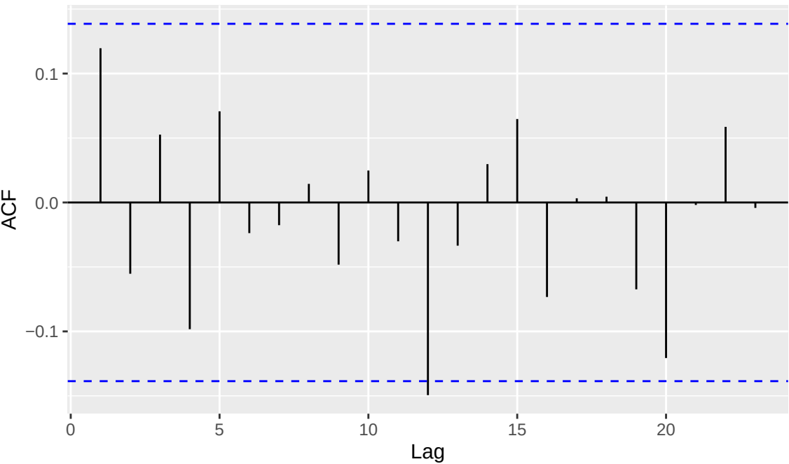
ACF, AR(1) \alpha=0.2
