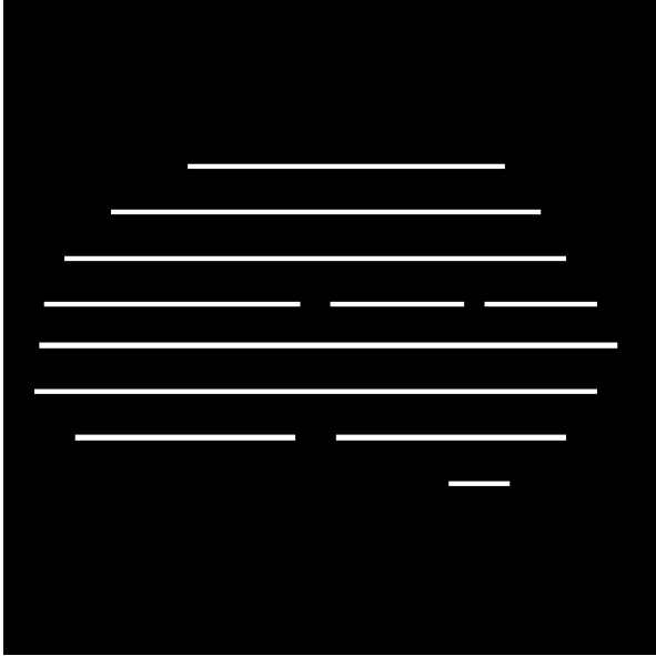
Known Mask
