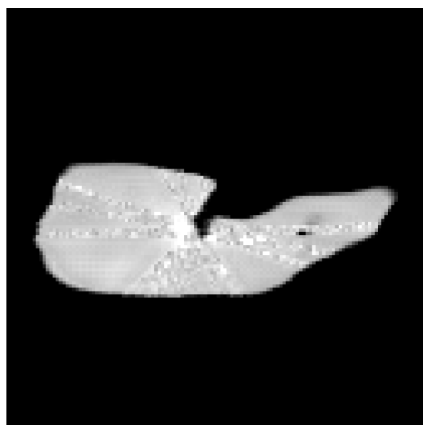
Hard-Constraint \hat{u}
