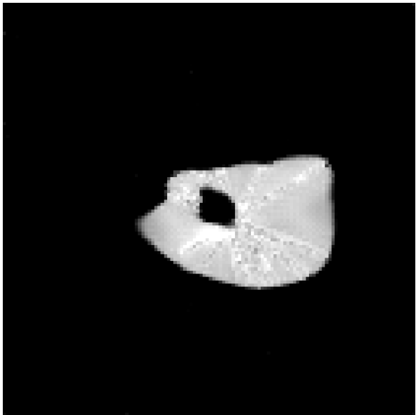
Hard-Constraint \hat{u}
