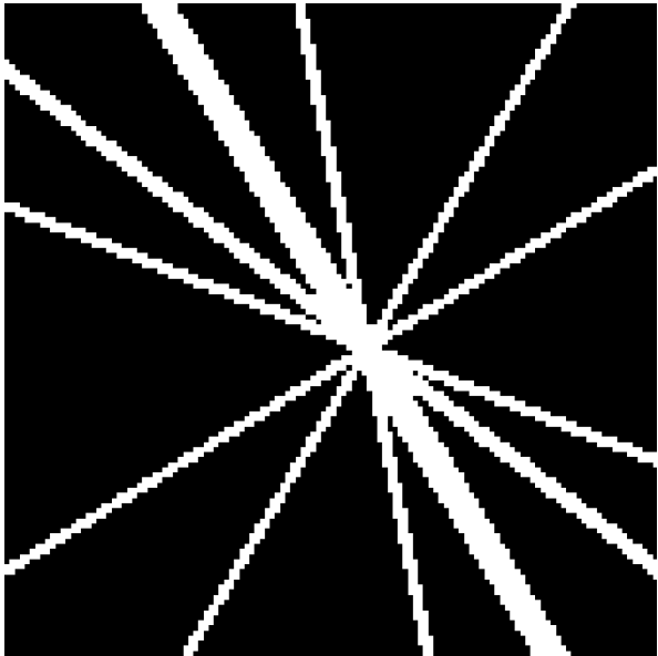
Known Mask
