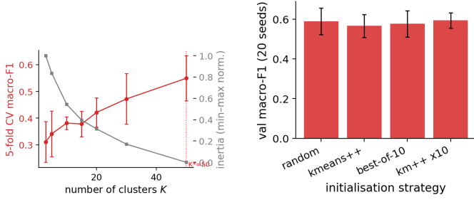
(a) K sweep: CV macro-F1 (red) and normalised inertia (grey). F1 keeps rising over the swept range; selected K=50 . (b) Init strategy at K=50 , 20 seeds each: better inertia does not translate to better F1.
