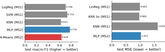
(a) Classification: test macro-F1 (higher = better). (b) Regression: test MSE (lower = better).
