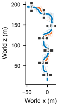
(a) Course 1: top view
