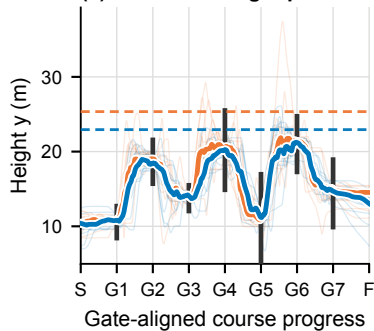
(c) Course 1: height profile
