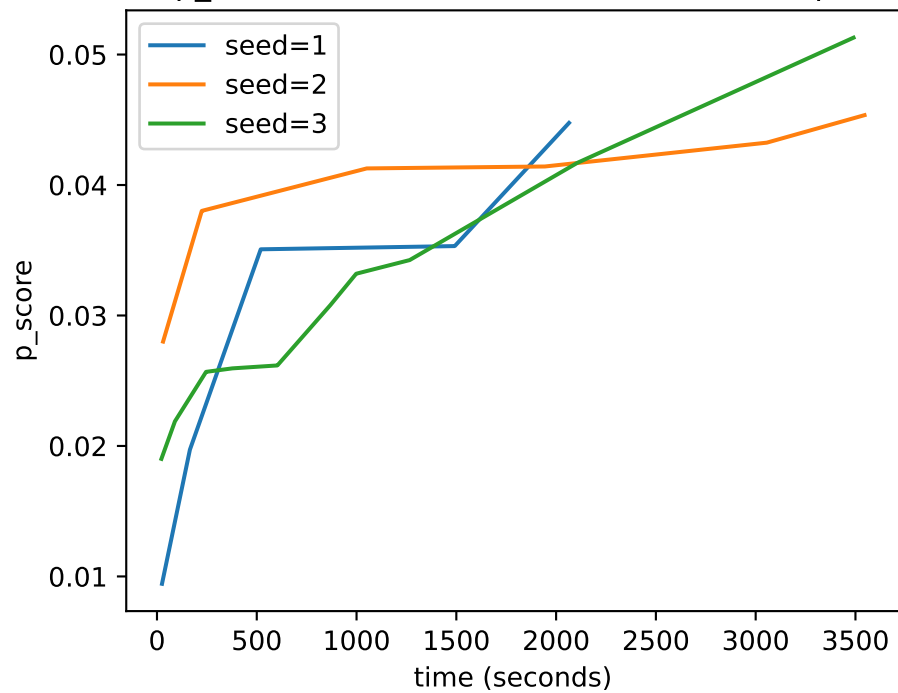
p_score vs time for cubic with 5 timesteps
