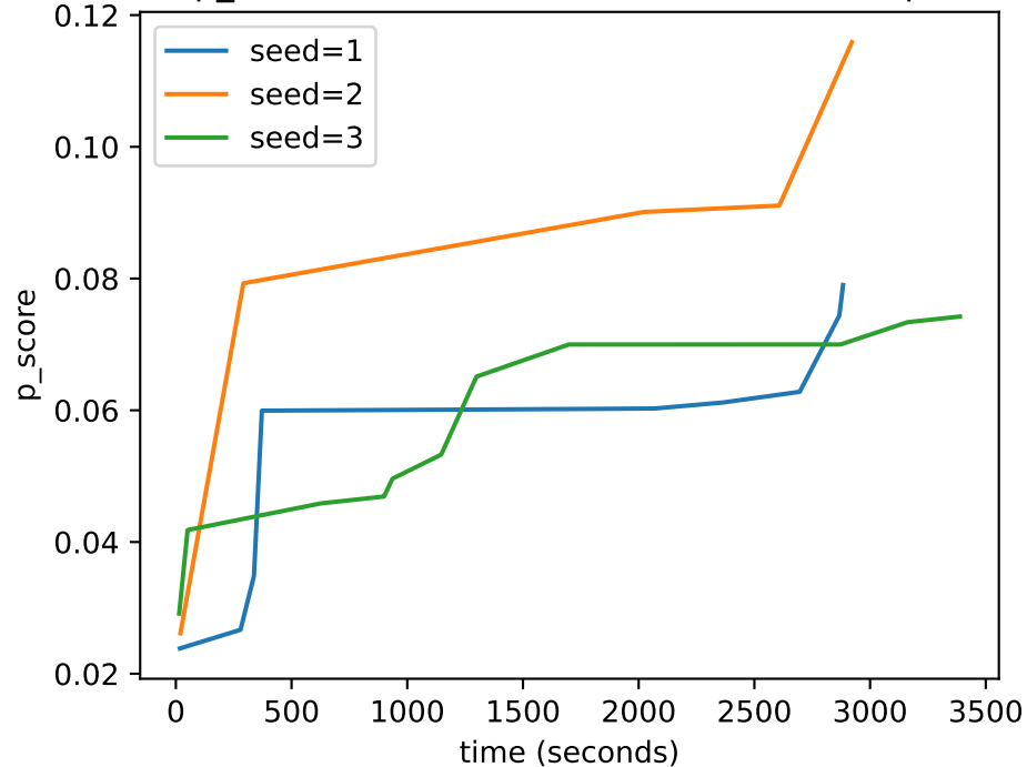
p_score vs time for cubic with 5 timesteps
