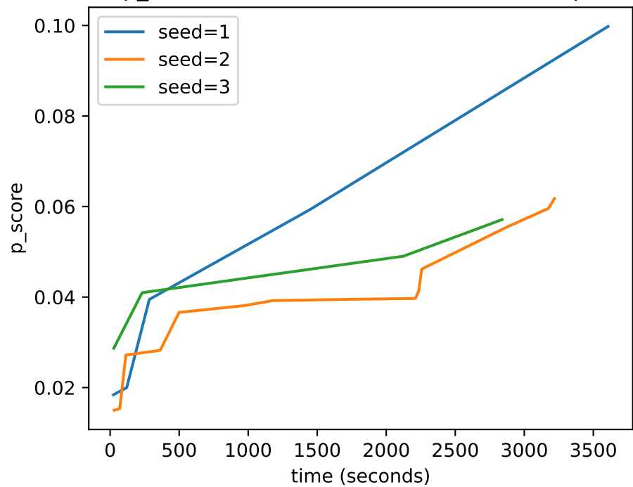
p_score vs time for cubic with 4 timesteps
