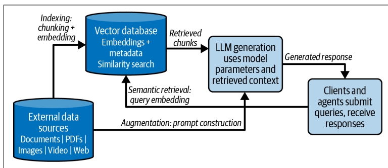
Figure 3-3. Dataflow in RAG apps
