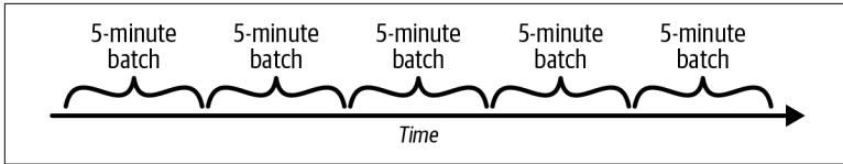
Figure 3-2. An example microbatch refresh
