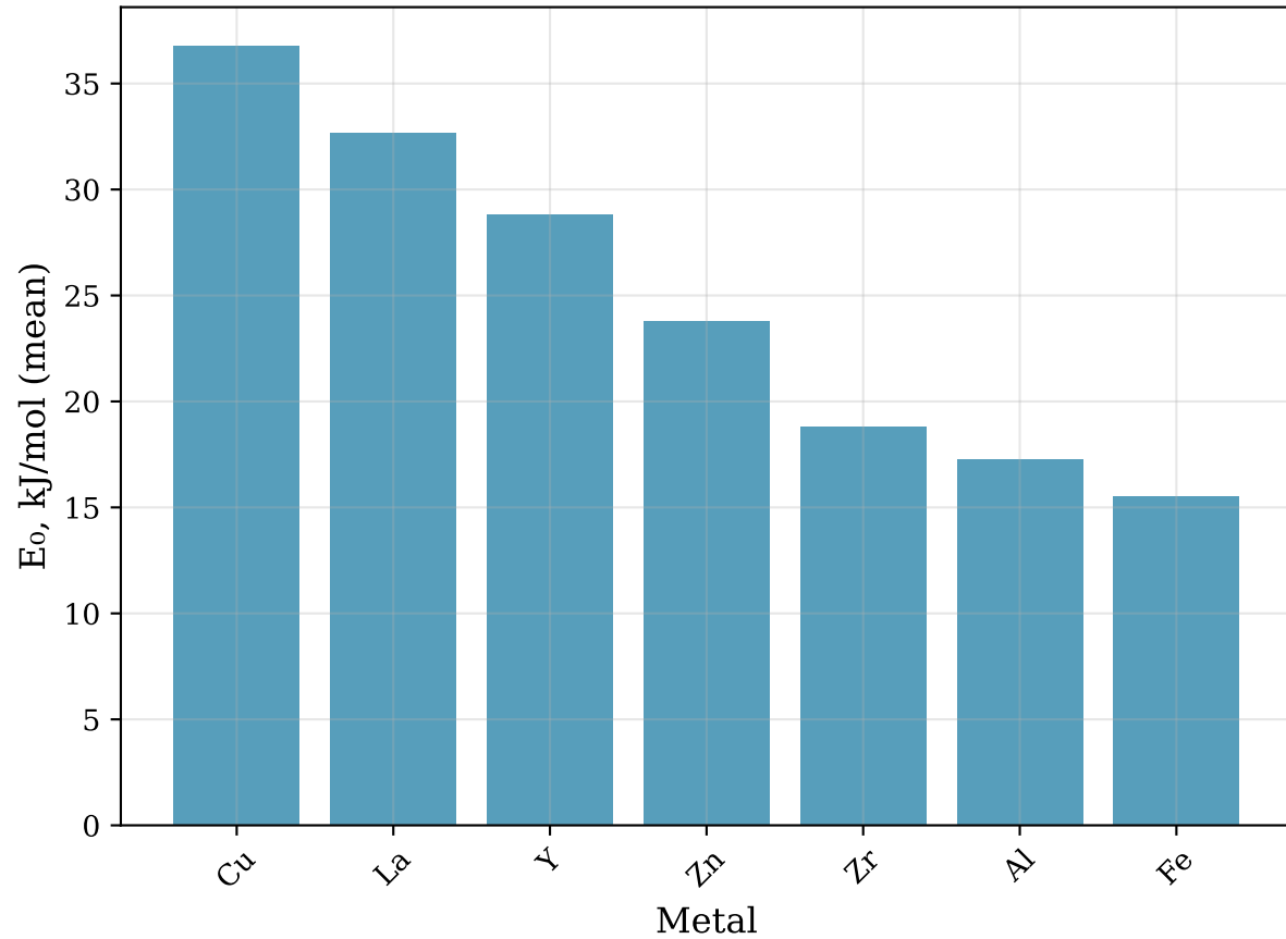
Characteristic Energy by Metal Type
