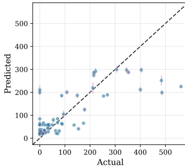
Sme, м2/г R^2=0.618 , RMSE=82.11
