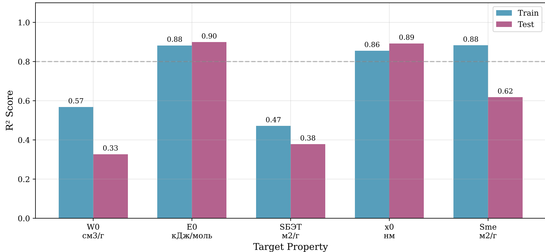
Forward Model Performance: Train vs Test R^2
