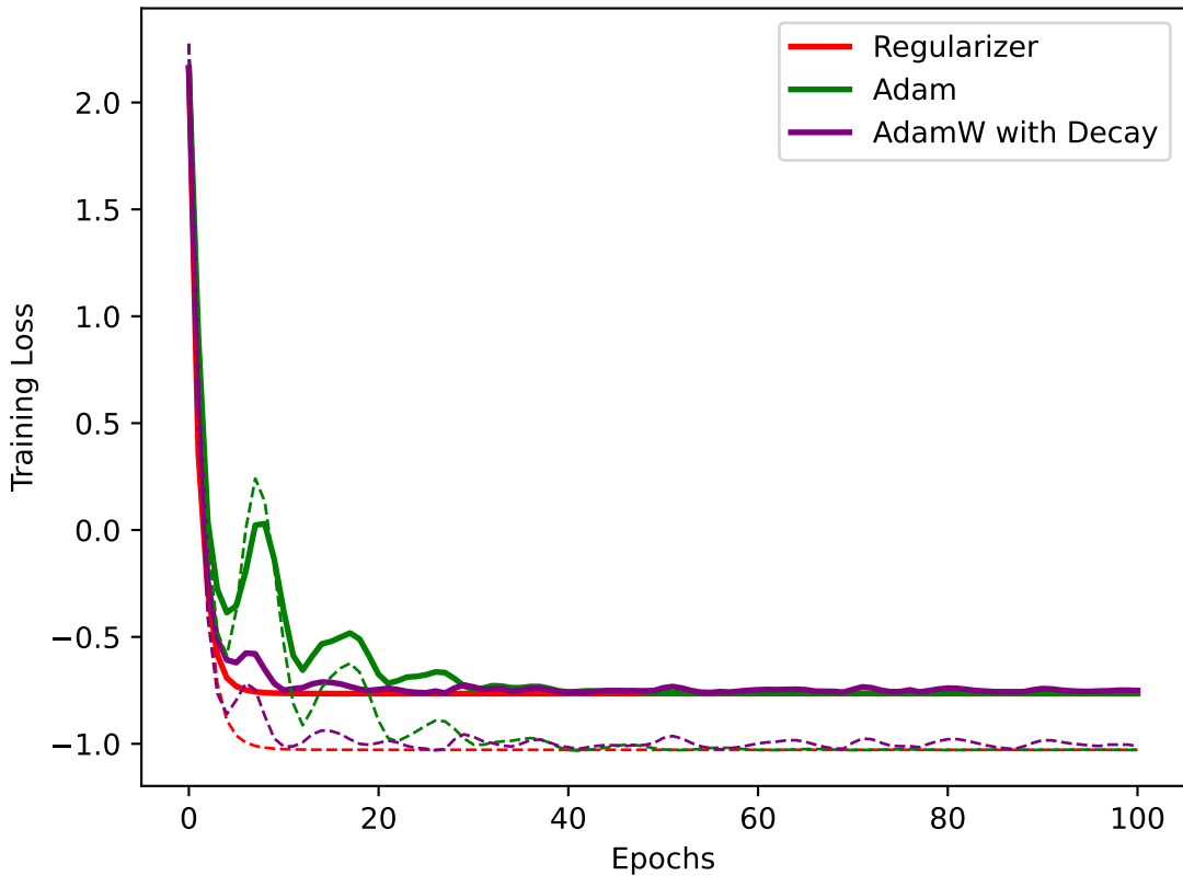
Loss curve of Poisson Regression
