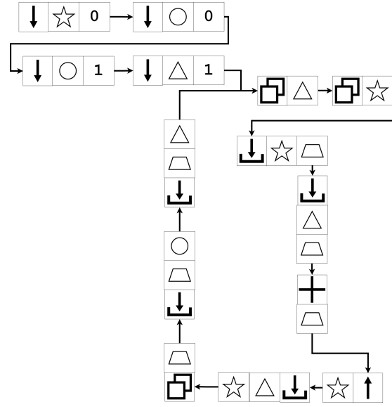
Figure 6.1: SCuLPT Fibonacci program
