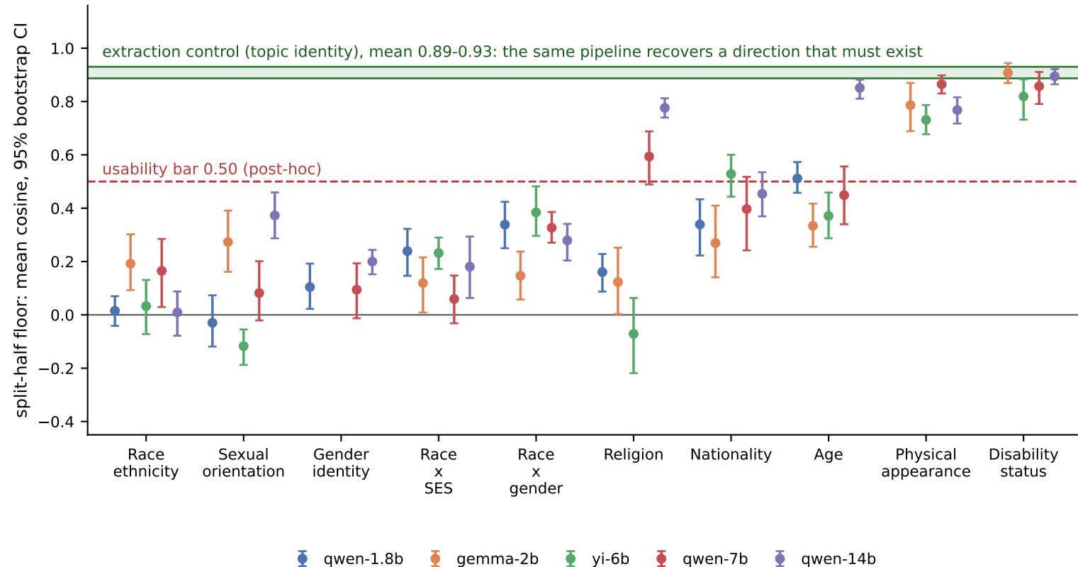
Every model-category floor, with its interval
