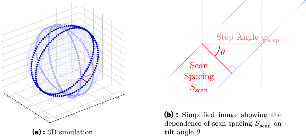
Figure 2.8: Visualisation of scan spacing on the tilt angle
