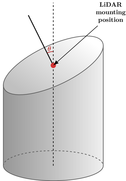
Figure 2.4: Proposed platform design. \theta is the tilt angle
