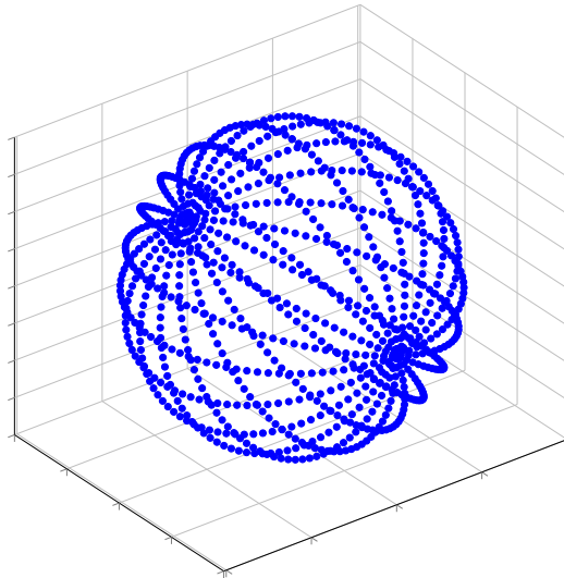
Figure 2.4: Simulation of an obtained point cloud using a tilting platform
