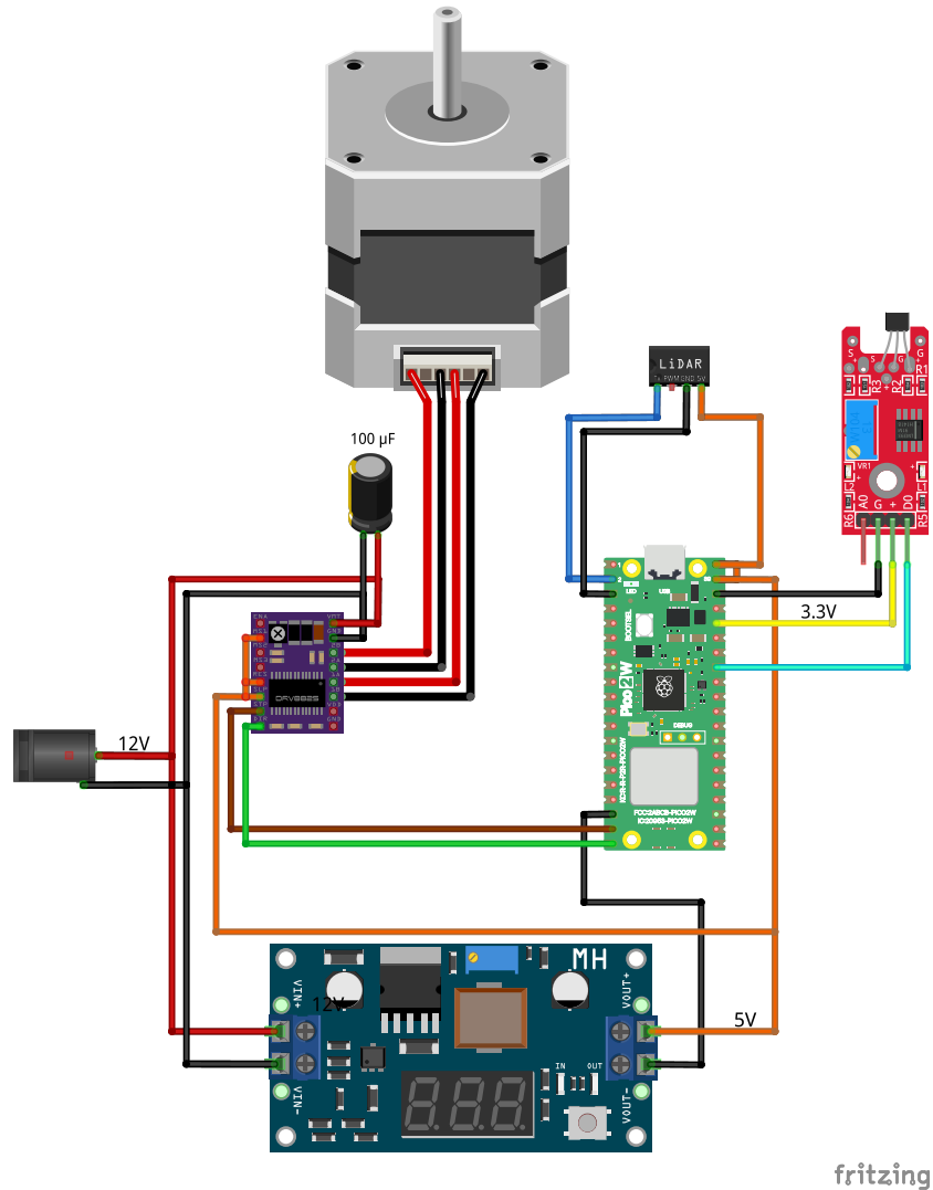
Figure 3.1: Wiring diagram of electronics 1
