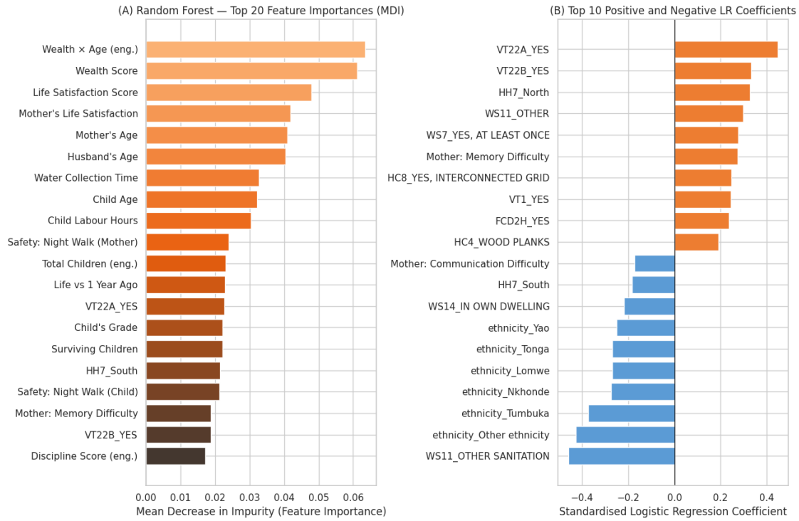
Figure 5: Model Interpretability — RF Importances and LR Coefficients
