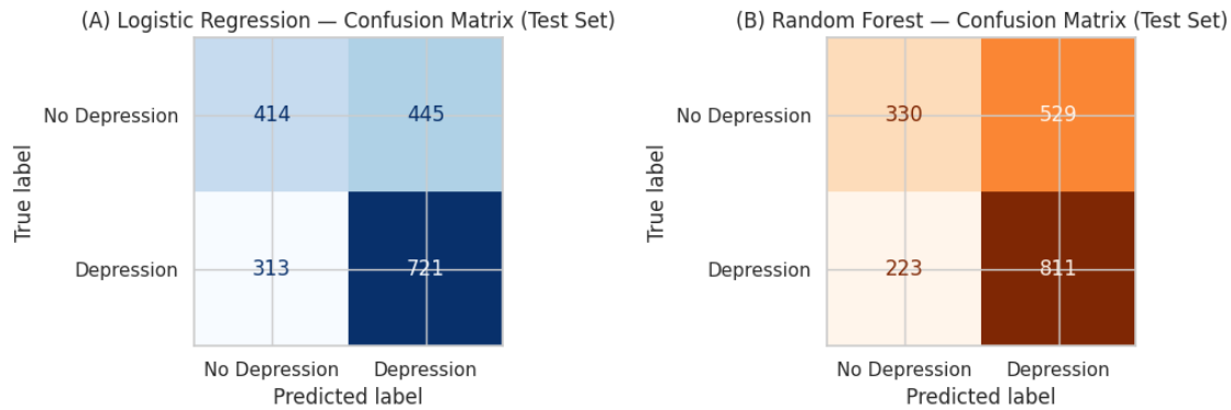
Figure 10: Confusion Matrices (Test Set, Default 0.5 Threshold)
