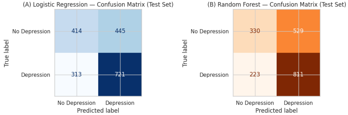
Figure 8: Confusion Matrices (Test Set, Default 0.5 Threshold)
