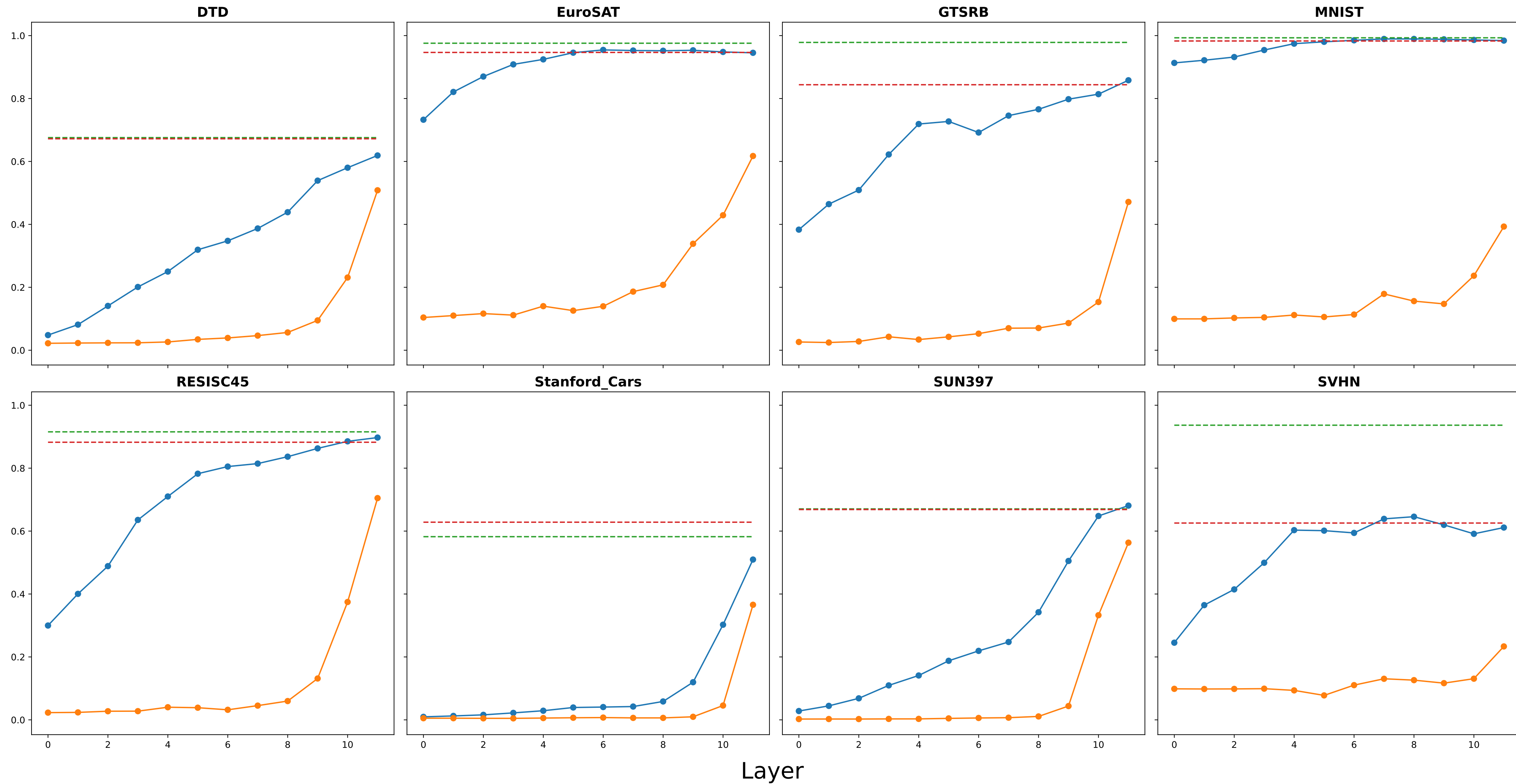
Classification Accuracy
