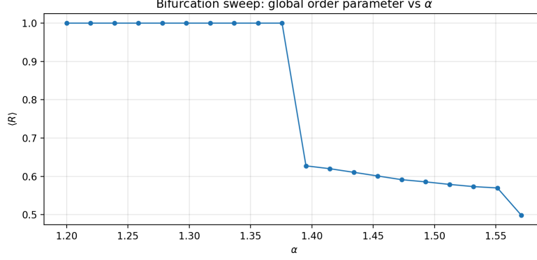
Figure 5: Bifurcation sweep: global order parameter \langle R \rangle vs. phase-lag \alpha .
