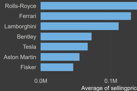
Average of sellingprice by make
