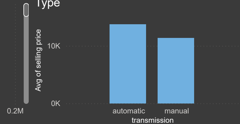
Avg of Selling Price By Transmission Type
