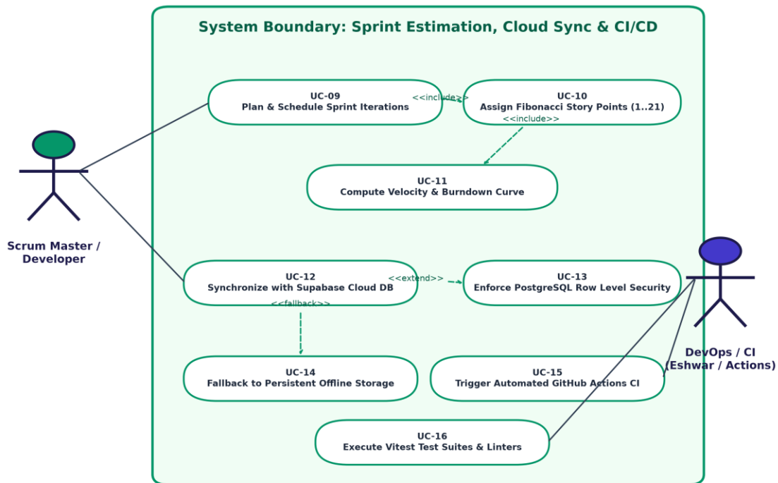
Figure 7.2: UML Use-Case Diagram — Agile Estimation, Cloud Database & CI/CD Subsystem
