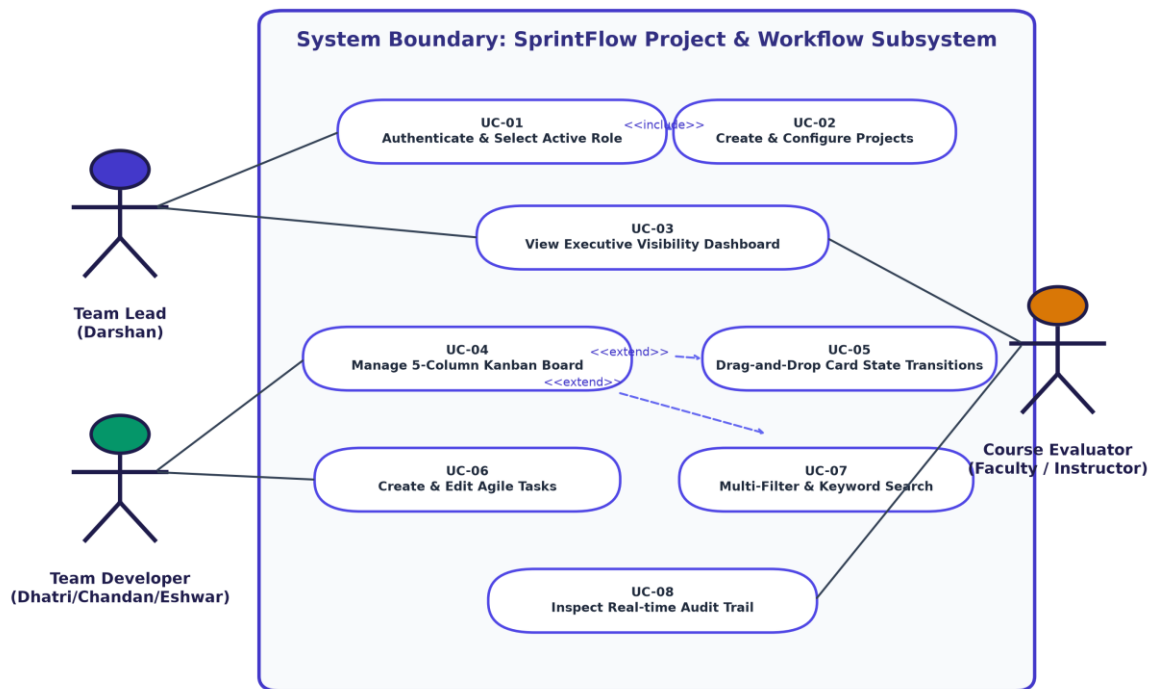
Figure 7.1: UML Use-Case Diagram — Project & Kanban Workflow Subsystem
