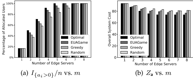
Fig. 3. Effectiveness vs. Number of Edge Servers (Set #1.2)
