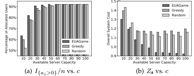
Fig. 7. Effectiveness vs. Available Server Capacities (#2.3)
