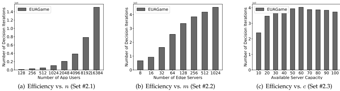
Fig. 8. Efficiency of EUAGame
