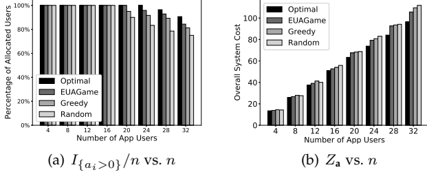
Fig. 2. Effectiveness vs. Number of App Users (Set #1.1)
