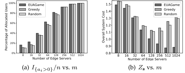
Fig. 6. Effectiveness vs. Number of Edge Servers (#2.2)
