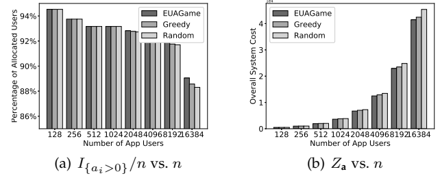
Fig. 5. Effectiveness vs. Number of App Users (Set #2.1)
