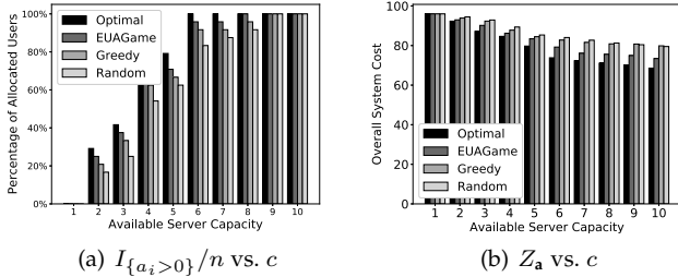
Fig. 4. Effectiveness vs. Server Computing Capacities (Set #1.3)
