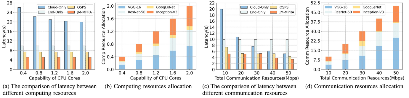
Fig. 16. Influence of total resources on latency and resources allocation proportion of different DNNs.
