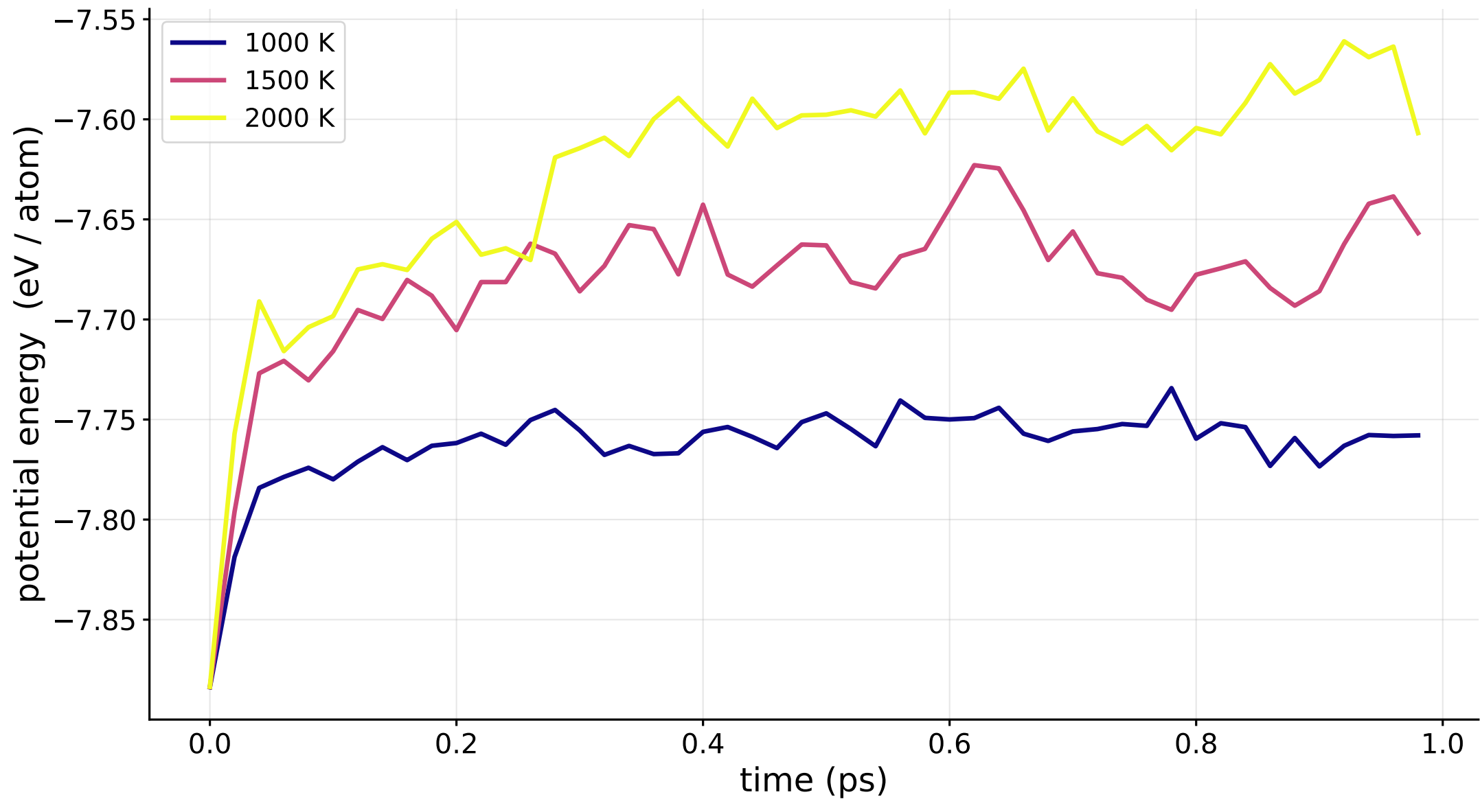
ISRU blend NVT MD — energy
