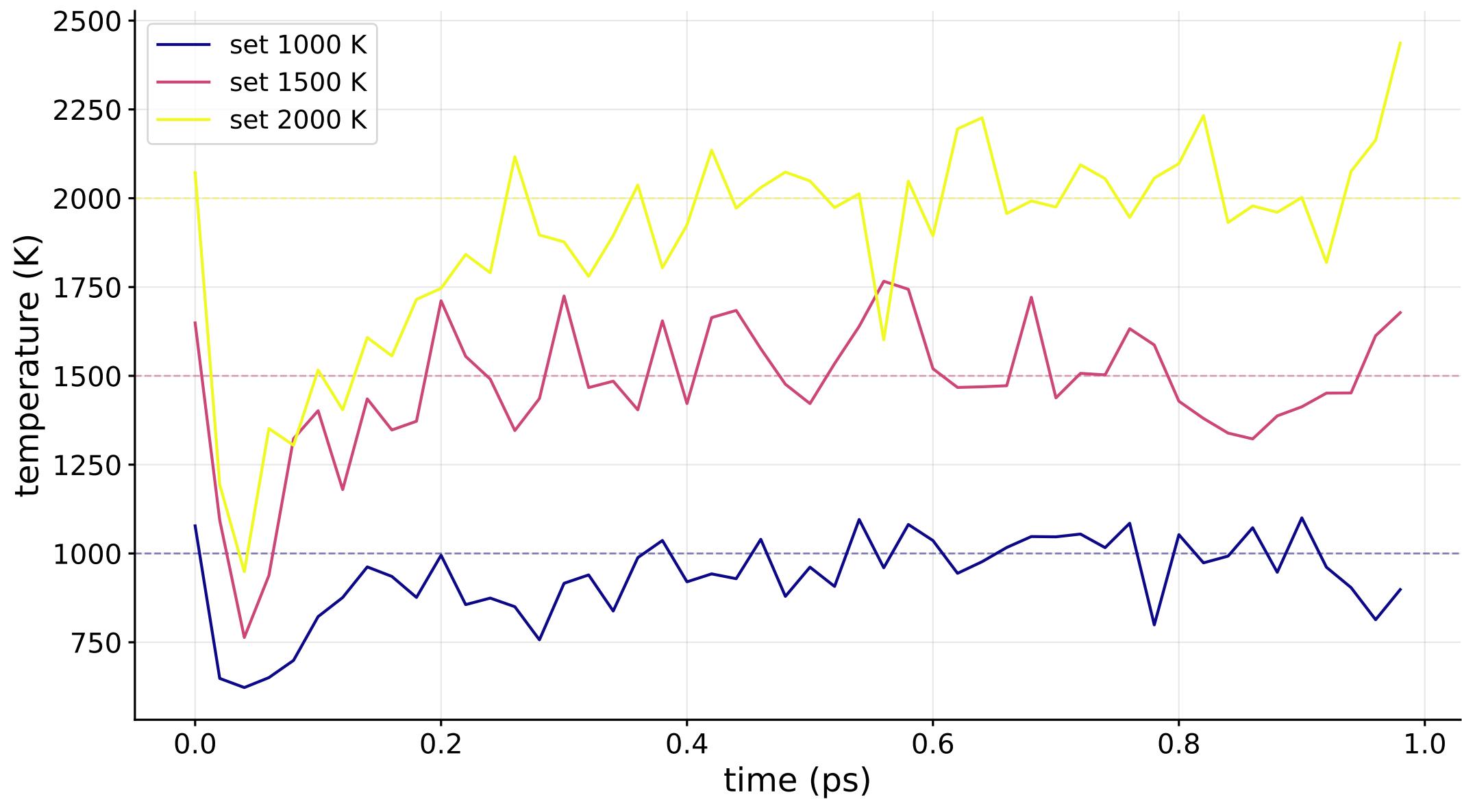
ISRU blend NVT MD — Langevin temperature equilibration
