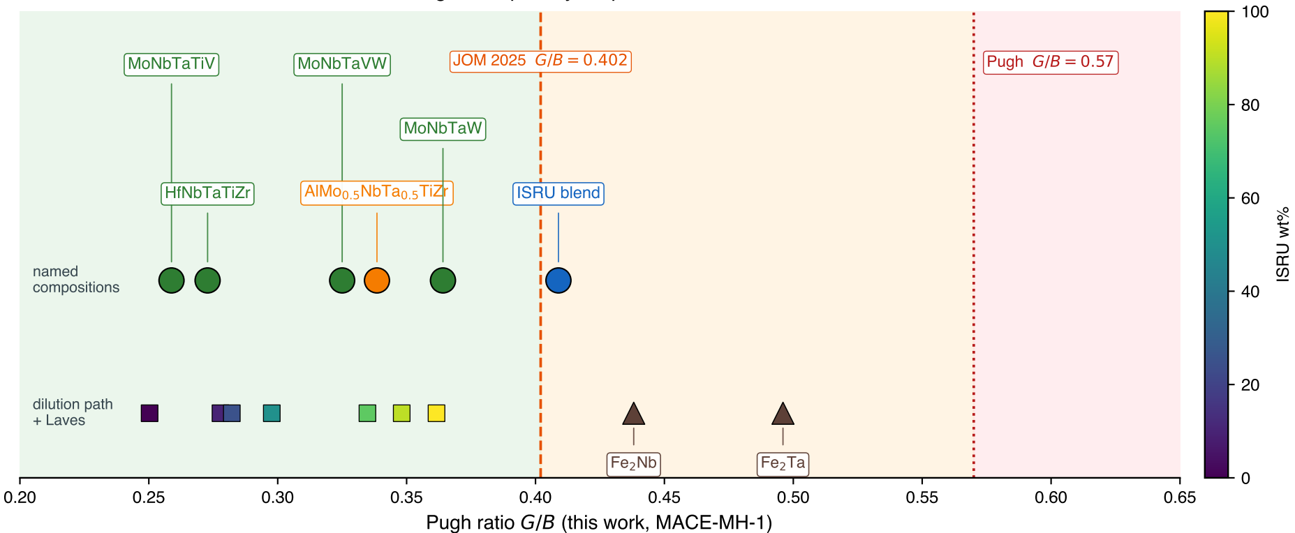
LPBF cracking-susceptibility map for SPARK-relevant RHEAs
