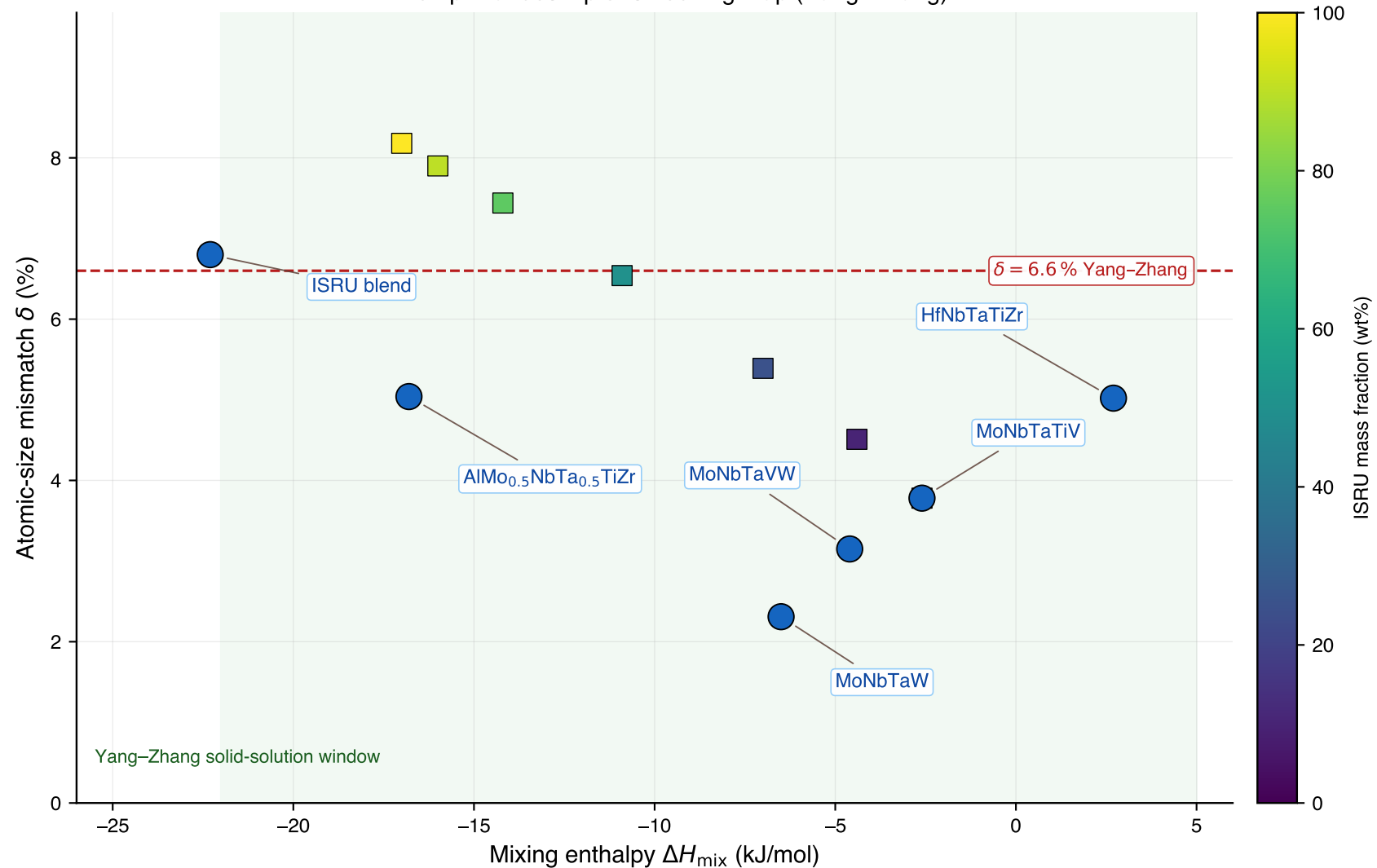
HEA empirical-descriptor screening map (Yang–Zhang)
