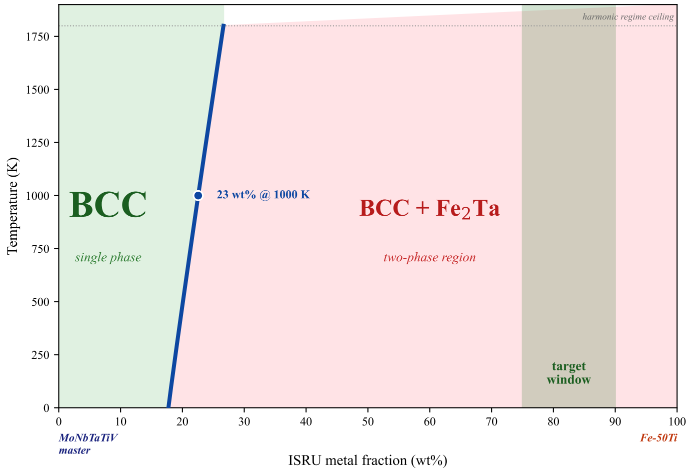
Tier-1 ab-initio dilution diagram (mace-mh-1 + harmonic phonons)
